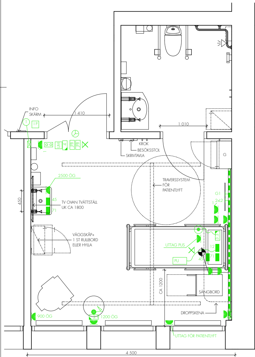
PLAN VÅRDRUM
